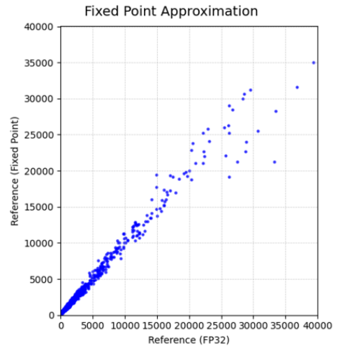
Figure 3: Fixed Point vs Floating Point
