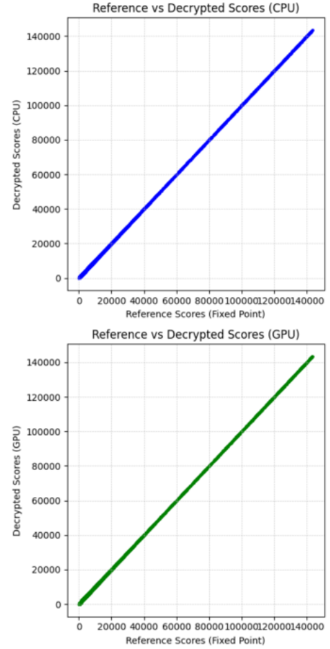
Reference (PlainText Fixedpoint) vs Decrypted Scores (CPU & GPU)
