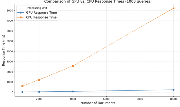
Figure 1: Python CPU vs Python GPU Answering Time
